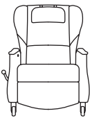
790-12, Treatment Chair W=31", D=42", H=48", SH=19 1/2", AH=26 1/2"
