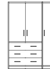
TENT/43, TV Wardrobe W=50", D=23½", H=72"
