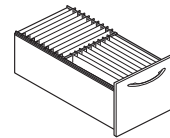
Legal - Side-to-Side 12" (304mm) Letter - Front-to-Back 9 3/4" (248mm)
