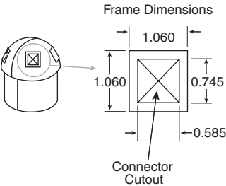
JAP-2 Data Connection Cutout Sizes
