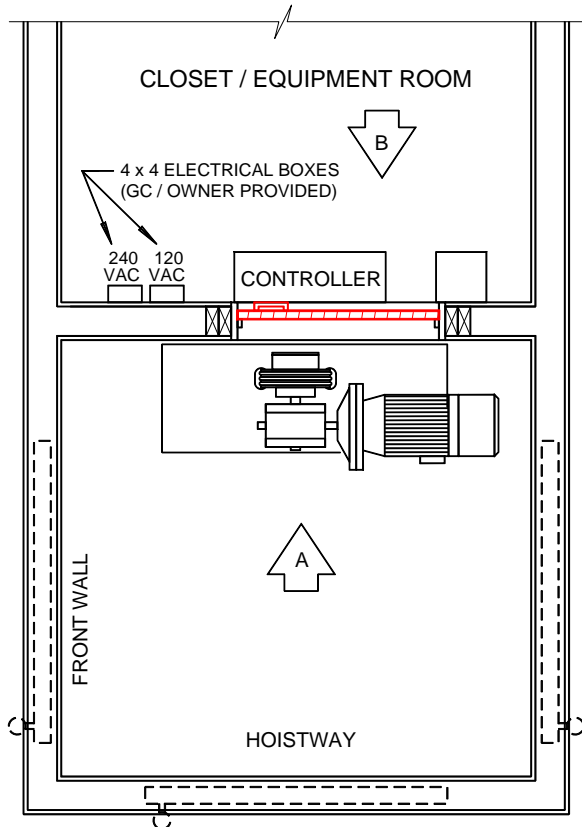
PLAN VIEW
