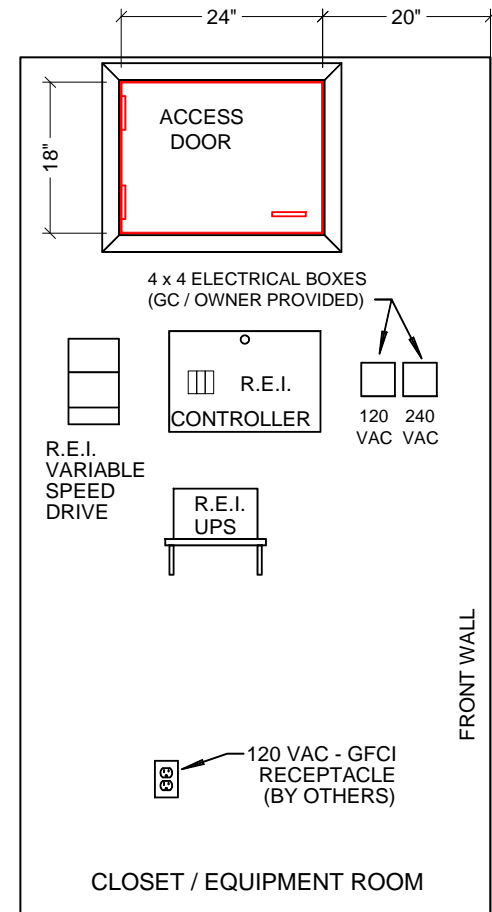
ELEVATION VIEW 'B'
