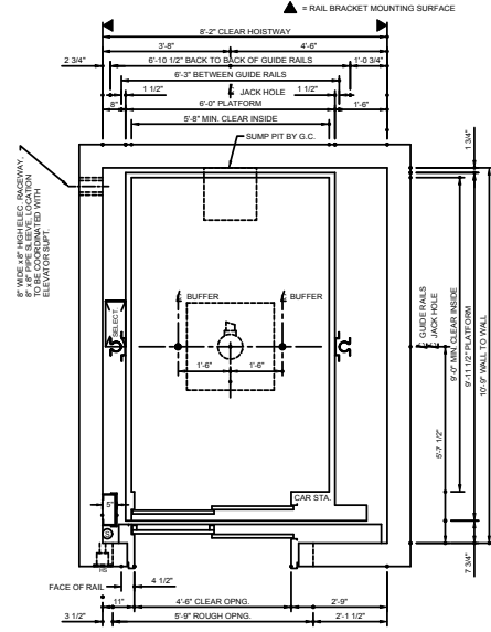
HOISTWAY PLAN
