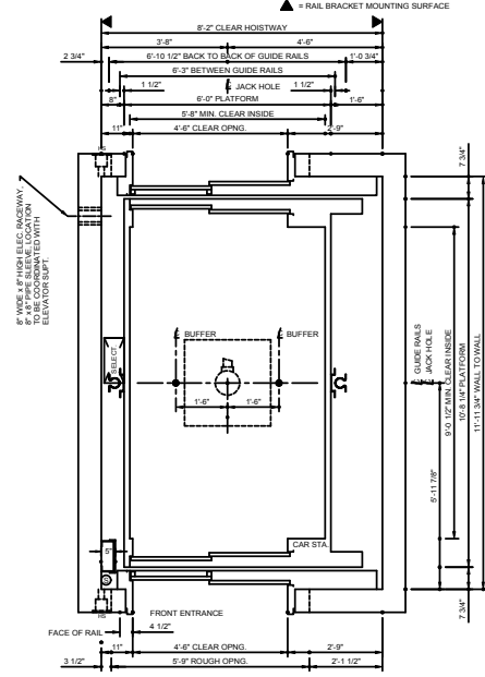
HOISTWAY PLAN
