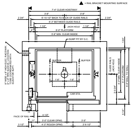
HOISTWAY PLAN
