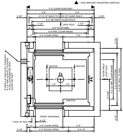
HOISTWAY PLAN NOTE: CONSULT ELEVATOR SUPP. FOR PIT BUMP LOCATION ON FRONT AND REAR ENTRANCE CAR.
