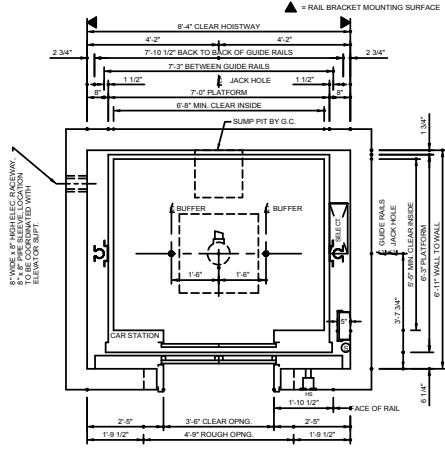
HOISTWAY PLAN
