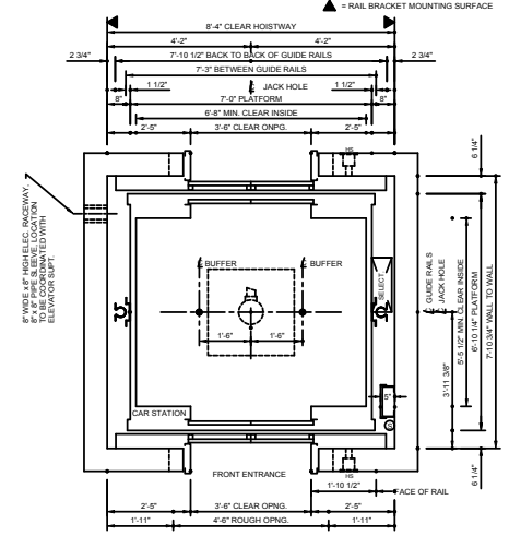
HOISTWAY PLAN NOTE: CONSULT ELEVATOR SUPP. FOR PIT BUMP LOCATION ON FRONT AND REAR ENTRANCE CARS.
