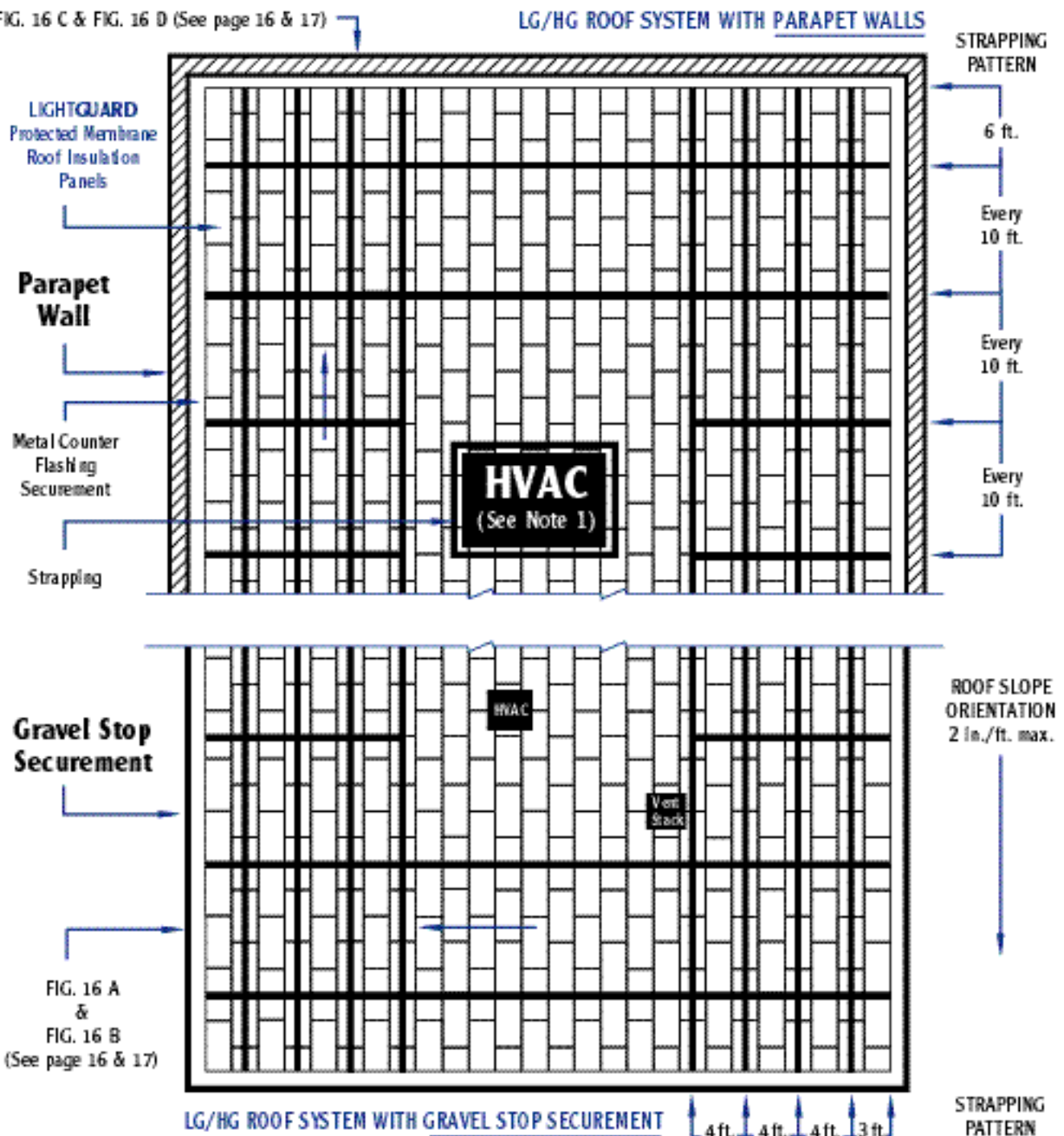
Figure 16 — System 3 Strapping Securement
