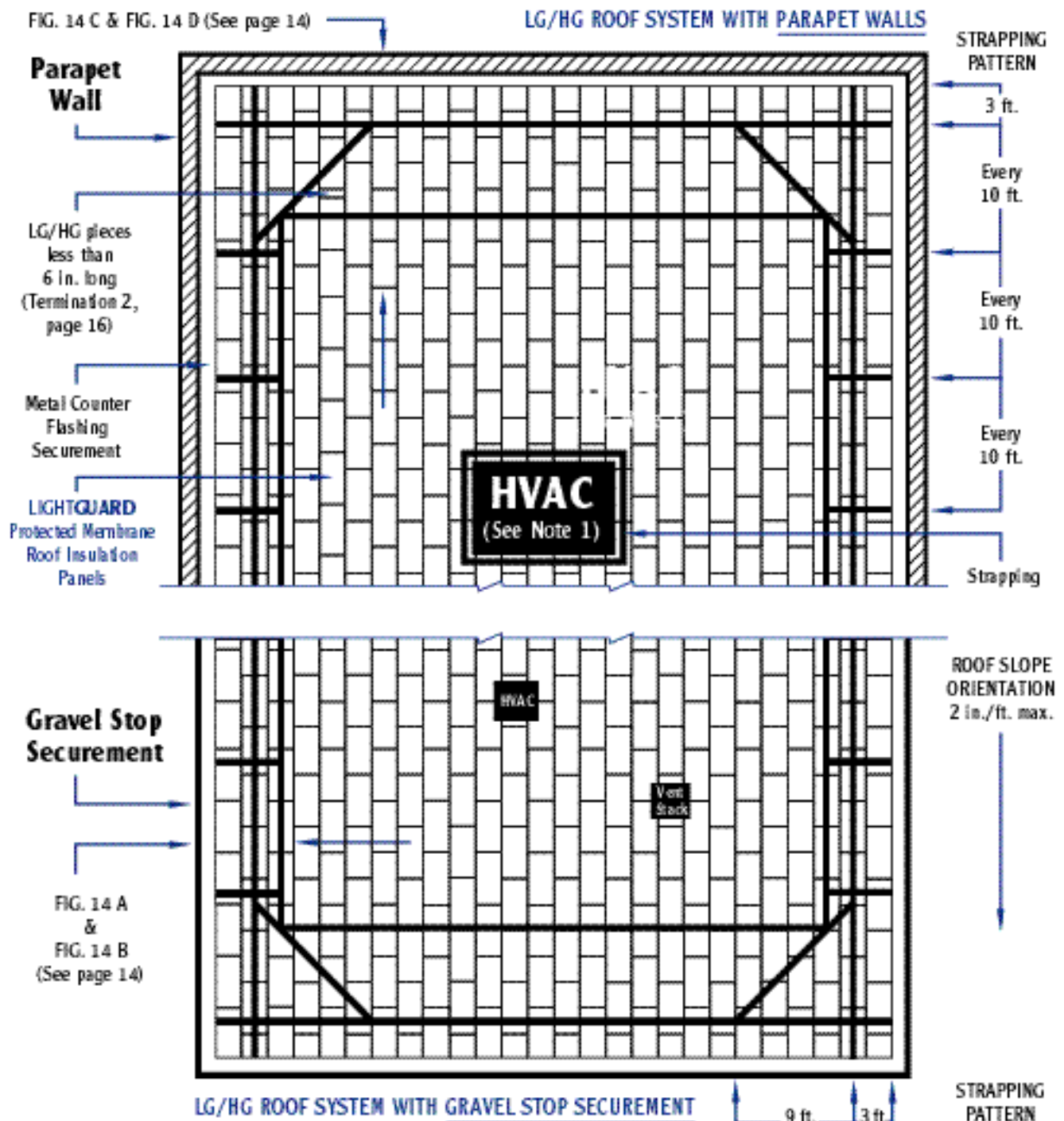
Figure 14 — System 2 Strapping Securement
