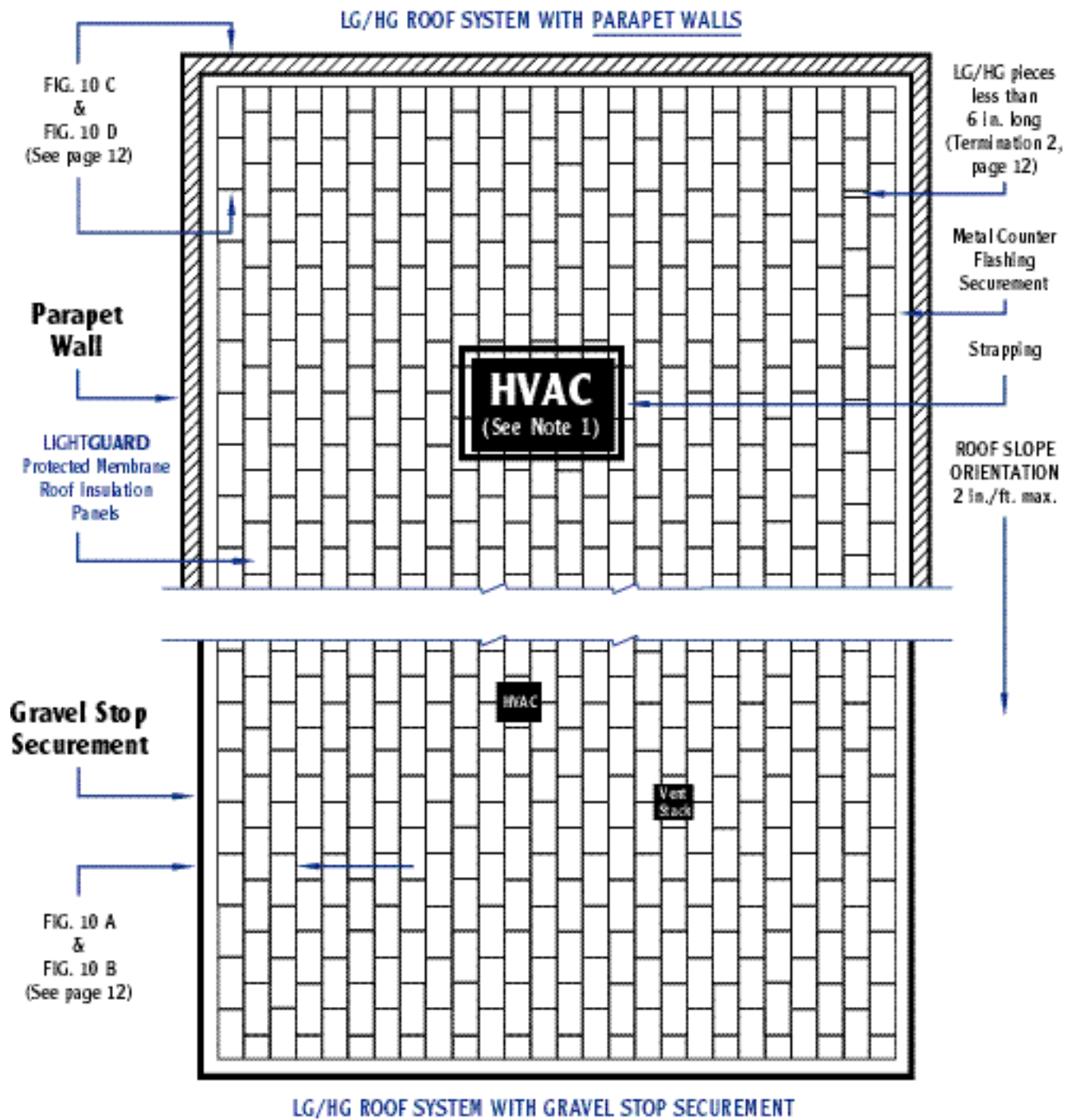
Figure 10 — System 1 Strapping Securement
