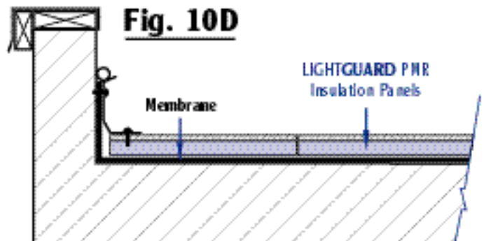
Detail Fig. 10D
