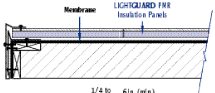
Detail Fig. 10B
