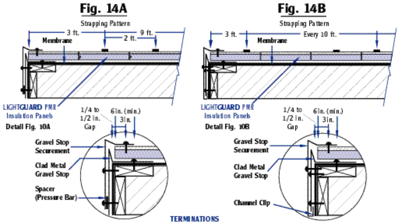
Figure 14A, 14B, 14C, 14D — System 2 Strapping Securement
