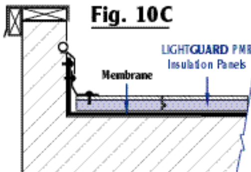
Detail Fig. 10C
