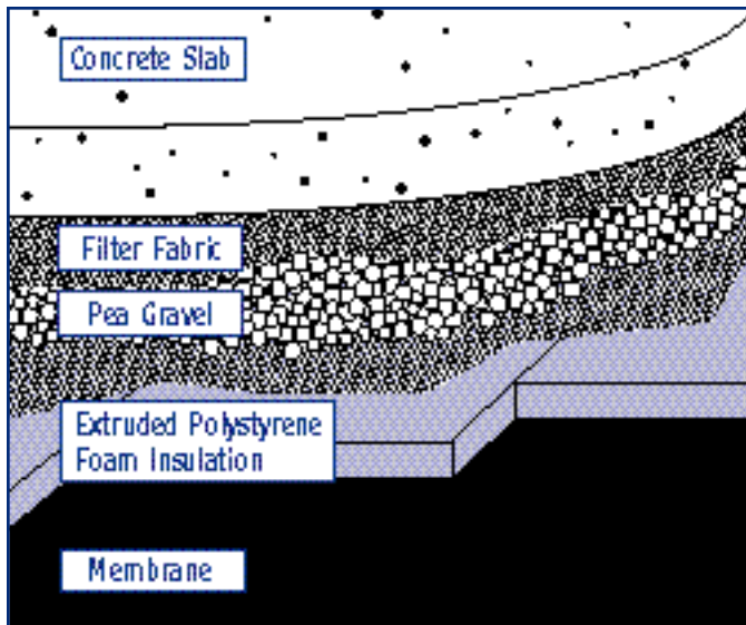
Figure 2. New Plaza Design
