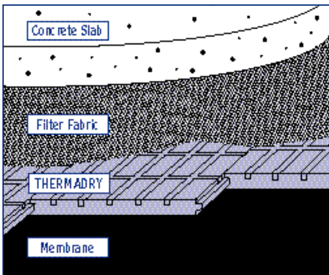
Figure 2. New Plaza Design
