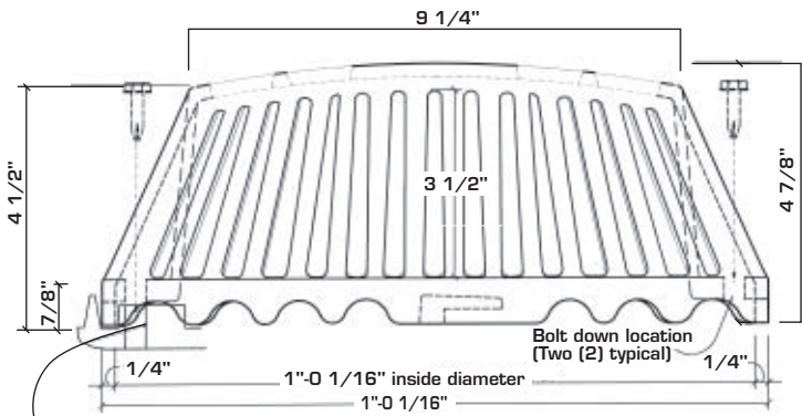
Strainer Elevation
