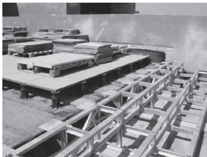
Public area - concrete tiles on Eterno pedestals
