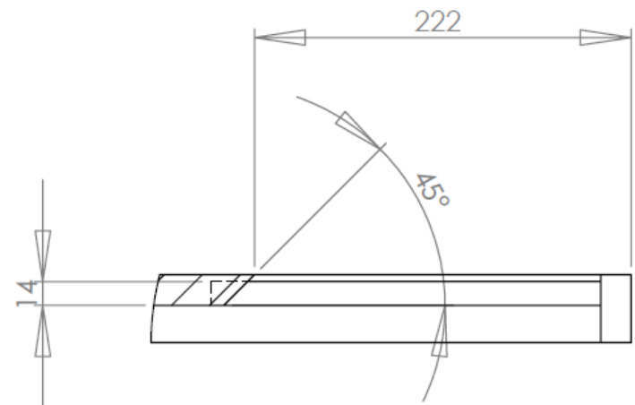
DETAIL D SCALE 1 : 5
