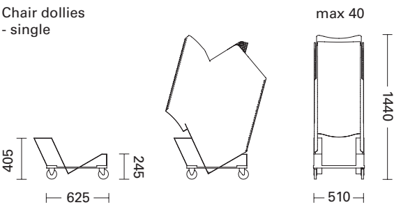
Chair dollies - double - triple - quadruple
