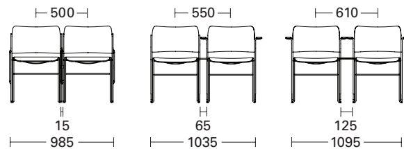
Side chairs - linked Armchairs - linked Side chair + armchair - linked
