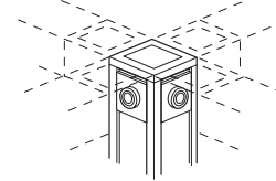
4-way 90° Post
