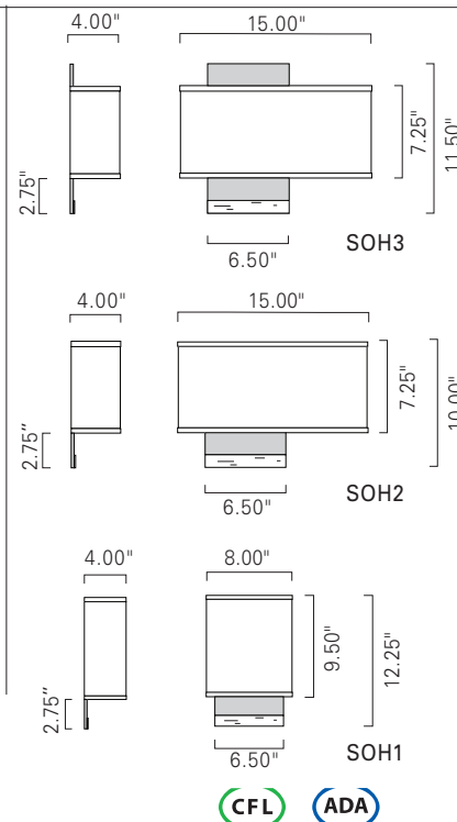
Soho Double Sconce SOH3 Brushed Aluminum Black Enamel BABL
