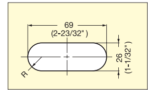
Bore Dimensions
