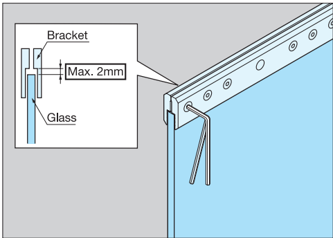
Mount bracket on corner and align to the edge of glass. Tightening Torque (clamp screw): 15N·m (132 lbs-in)
