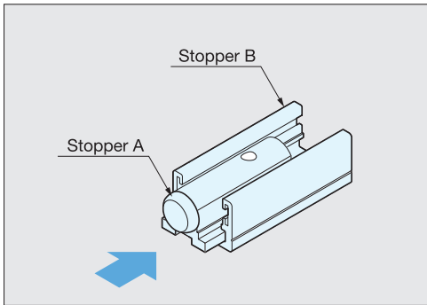
Install stopper B on floor and insert stopper A to B.
