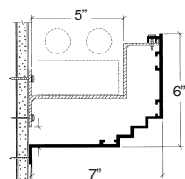
PROFILE #1086
