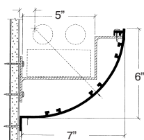
6" RADIUS PROFILE #1076
