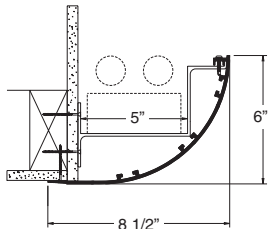
PROFILE #1066
