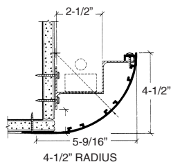
PROFILE #1066R
