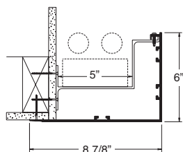
PROFILE #1106T
