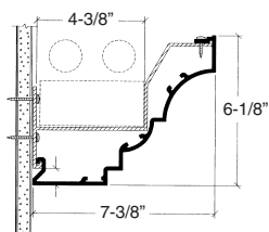
PROFILE #1096
