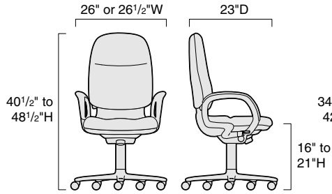
Work Chair Size II Adjustable High-Back
