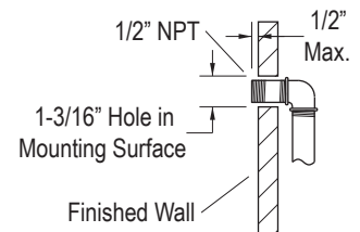
P23070 Installation Detail
