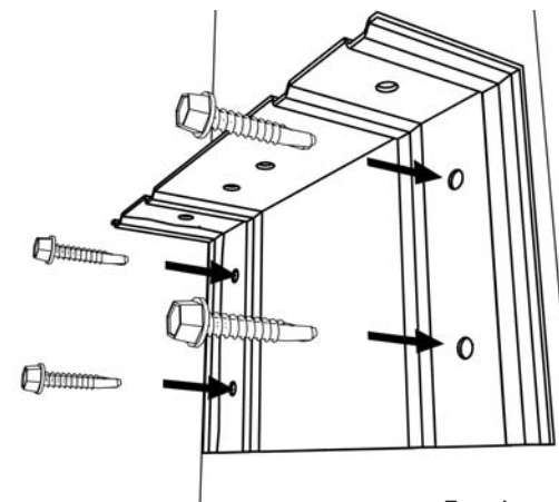
Framing Member
