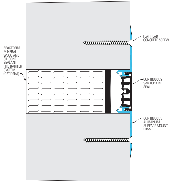
Reactofire Mineral Wool & Sealant Fire Barrier System (104-A07-050 system shown)
