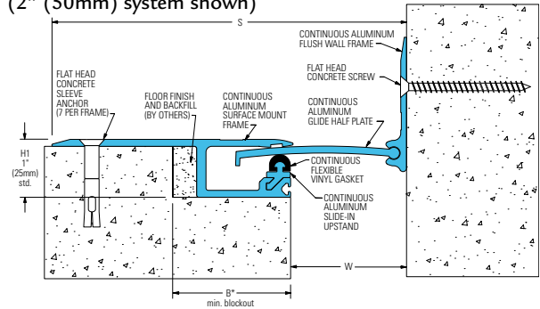
312-A02 Floor/Wall (2" (50mm) system shown)
