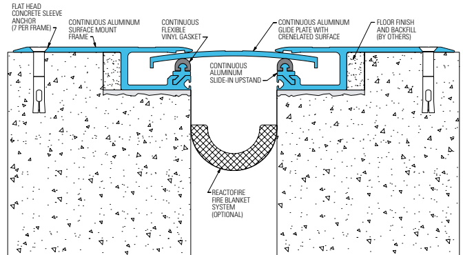
Reactofire Fire Blanket System (312-A01-050 system shown)
