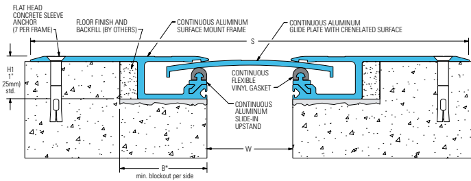
312-A01 Floor/Floor (2" (50mm) system shown)
