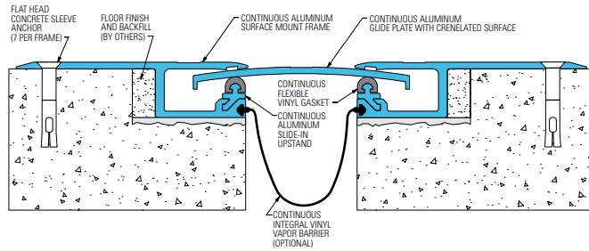
Integral Vapor Barrier (312-A01-050 system shown)
