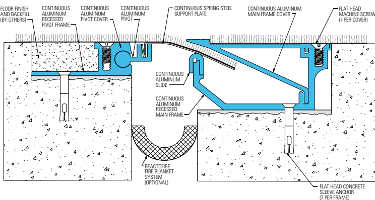
Reactofire Fire Blanket System (316-A01-050 system shown)
