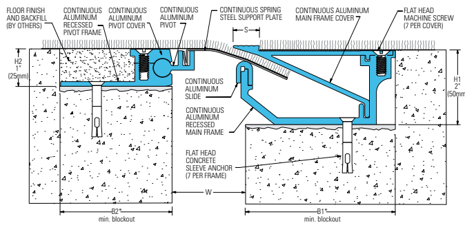
316-A01 Floor/Floor (2" (50mm) system shown)
