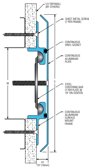
491-A07 Wall/Wall, Ceiling/Ceiling (4" (100mm) system shown)
