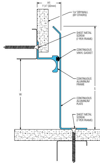
481-A09 Wall/Corner, Wall/Ceiling (4" (100mm) system shown)
