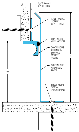
491-A09 Wall/Corner, Wall/Ceiling (4" (100mm) system shown)
