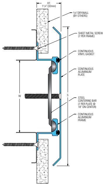
481-A07 Wall/Wall, Ceiling/Ceiling (4" (100mm) system shown)
