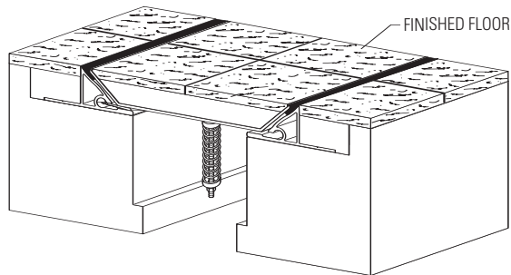
Fig. 4 (501-A01 completed installation)
