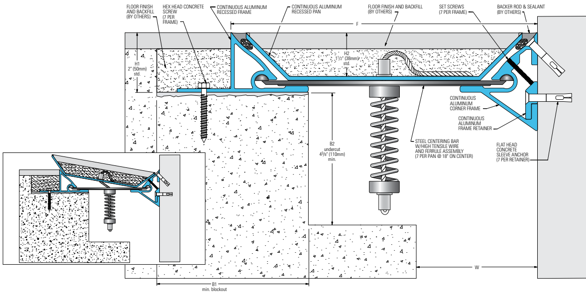
501-A02 Floor/Wall (4” (100mm) system shown)
