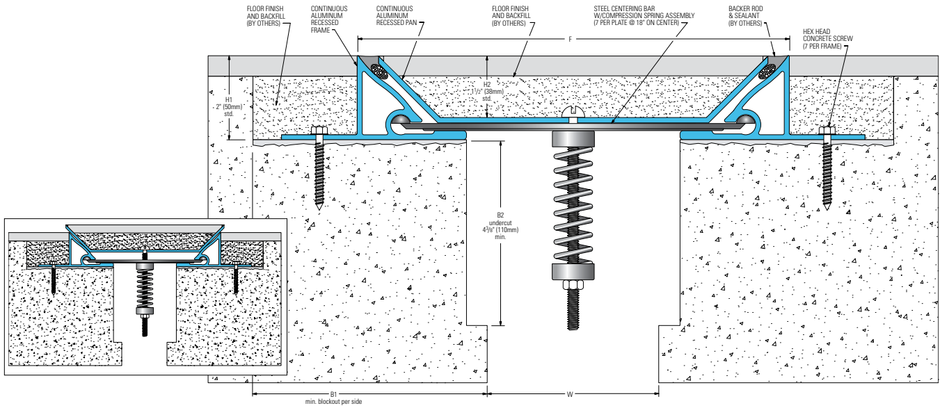
501-A01 Floor/Floor (4” (100mm) system shown)
