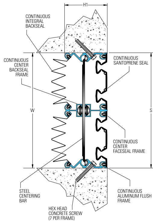
616-A07 Wall/Wall Ceiling/Ceiling (8" (200mm) system shown)
