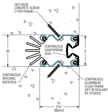
615-A07 Wall/Wall Ceiling/Ceiling (2" (50mm) system shown)
