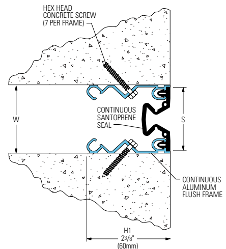
611-A07 Wall/Wall Ceiling/Ceiling (2" (50mm) system shown)
