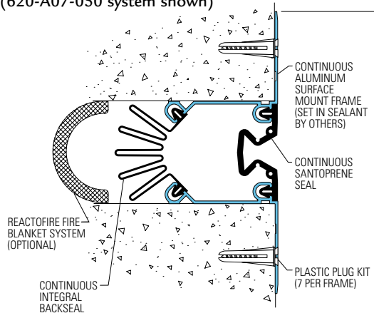
Reactofire Fire Blanket System (620-A07-050 system shown)
