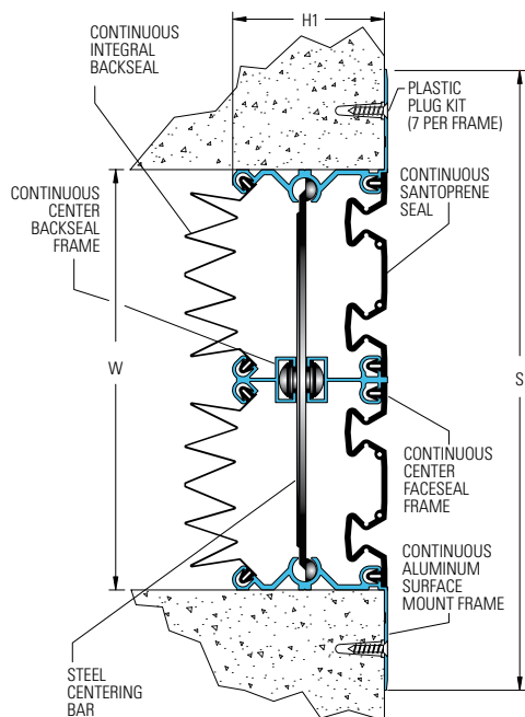
621-A07 Wall/Wall (8" (200mm) system shown)
