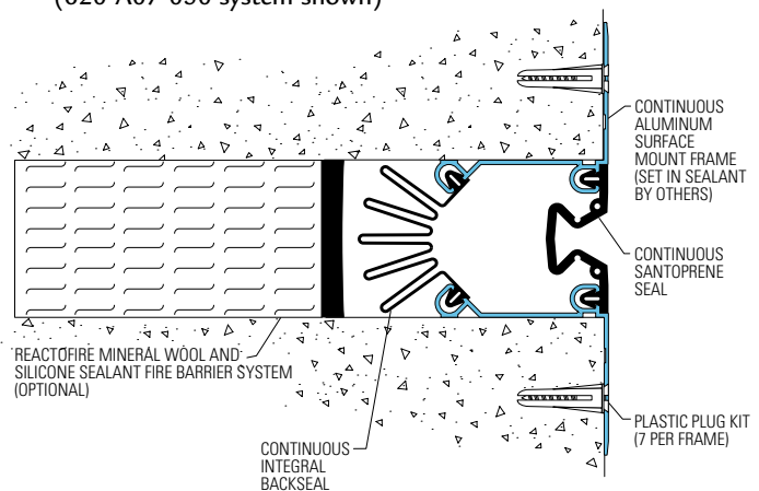
Reactofire Mineral Wool & Sealant Fire Barrier System (620-A07-050 system shown)
