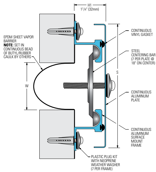
651-A07 Wall/Wall Ceiling/Ceiling (2" (50mm) system shown)
