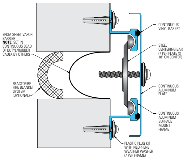
Reactofire Fire Blanket System (651-A07-050 system shown)
