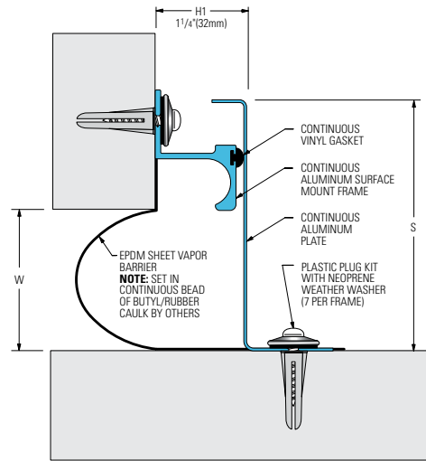
651-A09 Wall/Corner Wall/Ceiling (2" (50mm) system shown)
