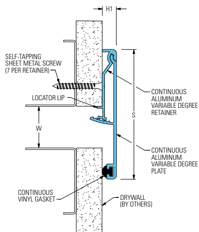
811-A07 Wall/Wall Ceiling/Ceiling (1" (25mm) system shown)
