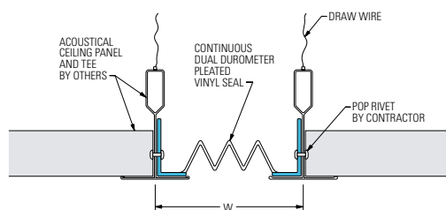
821-V24 Ceiling/Ceiling (2" (50mm) system shown)
