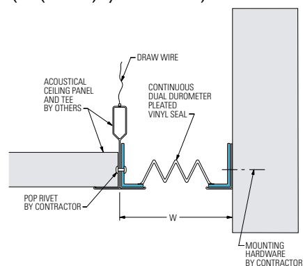
821-V23 Wall/Ceiling (2" (50mm) system shown)
