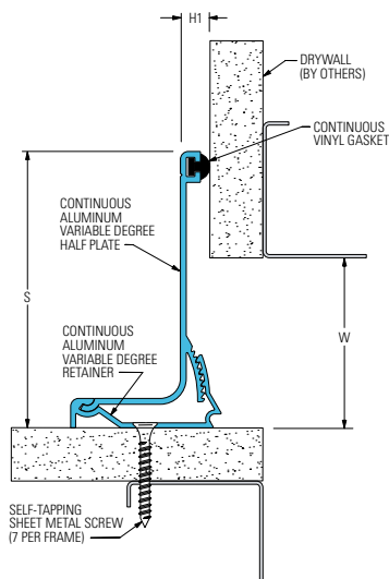
811-A09 Wall/Corner Wall/Ceiling (2" (50mm) system shown)
