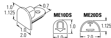
1" / 2" Quick Stop End Cap
