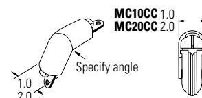
1" / 2" Snap-on Custom Angle Corner
