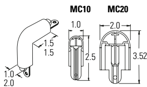
1" / 2" Snap-on 90° Outside Corner
