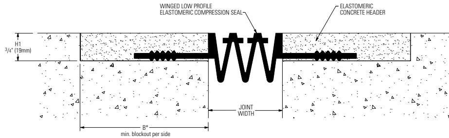
WM Series Deck/Deck (2" (50mm) system shown)
