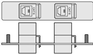
Data Architectural Adapter Plate has two CAT 6 RJ45 barrel (pass-through) outlets.
