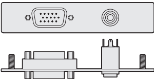
Video/Audio Architectural Adapter Plate has one VGA outlet (HD15 female to female gender changer) and one audio outlet (3 1/2 mm stereo mini jack to solder tabs).
