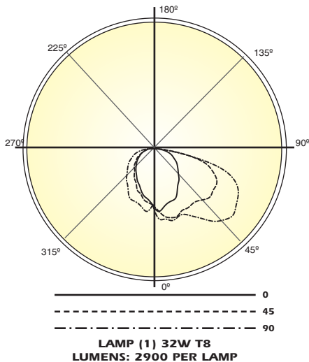
Candela Distribution:
