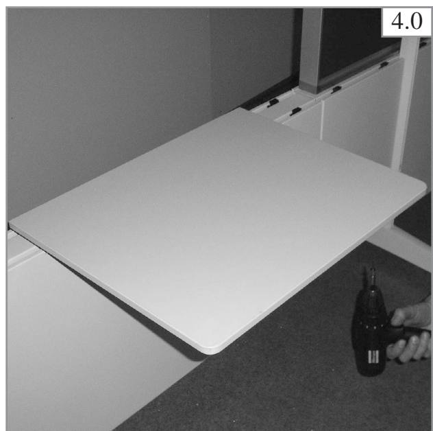
Druckerboard an Boardträger anschrauben. Screw printer board on to board brackets. Visser la desserte sur les supports.
