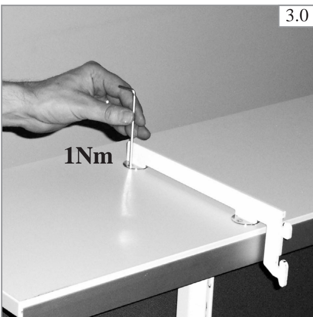
Boardträger fixieren. Fasten board brackets. Visser les supports.
