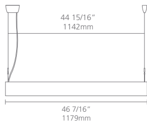
SINGLE SUSPENSION
