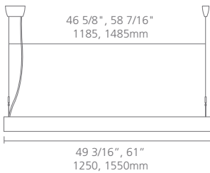
SINGLE SUSPENSION
