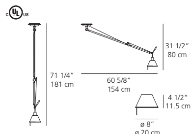
Tolomeo off-center suspension (aluminum diffuser)
