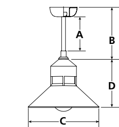
AA-30-P13.25"/AA-31-P13.25"
