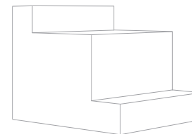
Three-Tier 34"H x 36"W x 40"D Top Tier 8½"H x 10"D Middle Tier 16"H x 18"D Bottom Tier 9½"H x 12"D
