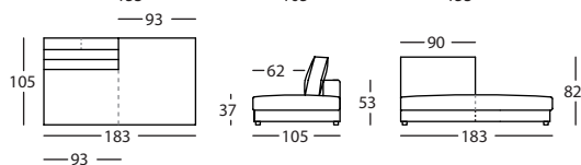
243.17.LU.6.D RIGHT TERMINAL MODULE 183 WOODEN FEET
