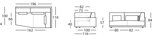
256.16.VJ.Q.D RIGHT STRAIGHT CORNER 196 DOUBLE DEPTH HIGH 84
