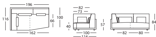
256.16.VJ.Q.I LEFT STRAIGHT CORNER 196 DOUBLE DEPTH HIGH 84
