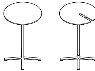
236/3 Ø 70 (27 1 / 2 "), H 105 (41 3 / 8 ")
