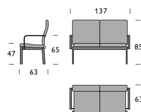
Modell 4082 / 4085 Weight ~ 20 kg
