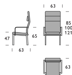
Model 4040 / 4045 / 4048 Weight 9.6 / 10.5 / 11.0 kg
