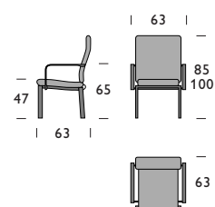
Model 4040 / 4045 Weight 9.8 / 10.5 kg
