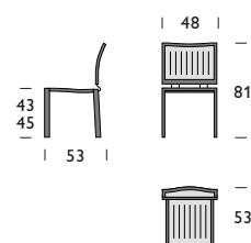
Model 4001
