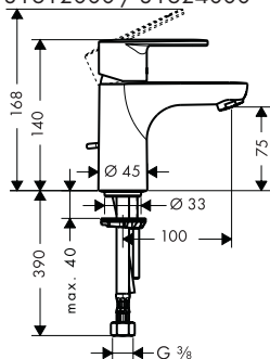
Talis E 2 31612000 / 31624000
