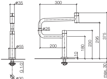
17 800 875 POT FILLER Cold-water valve, 19 5/8" spout projection Rubinetto acqua fredda, sporgenza 19 5/8" Válvula de agua fría, saliente 19 5/8"
