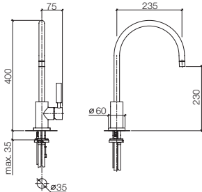
33 815 888 Single-lever mixer, 9 1/4" spout projection Miscelatore monocomando, sporgenza 9 1/4" Mezclador monomando, saliente 9 1/4"
