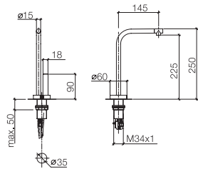
17 851 790 / 17 850 790 Hot & Cold/Hot Water Dispenser, 5 3/4" spout projection Hot & Cold/Hot Water Dispenser, sporgenza 5 3/4" Hot & Cold/Hot Water Dispenser, saliente 5 3/4"
