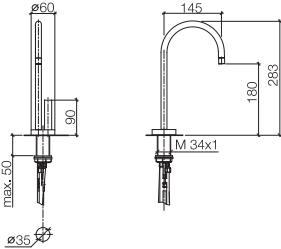
17 851 875 / 17 850 875 Hot & Cold/Hot Water Dispenser, 5 3/4" spout projection Hot & Cold/Hot Water Dispenser, sporgenza 5 3/4" Hot & Cold/Hot Water Dispenser, saliente 5 3/4"
