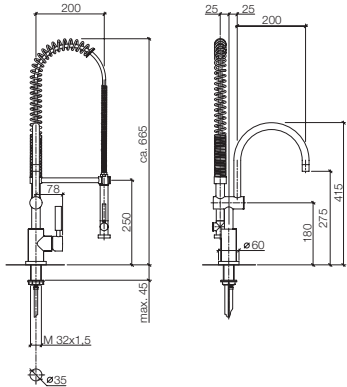
33 880 888 Profi single-lever mixer, 9 1/4" spout projection Miscelatore monocomando professionale, sporgenza 9 1/4" Mezclador monomando profesional, saliente 9 1/4"
