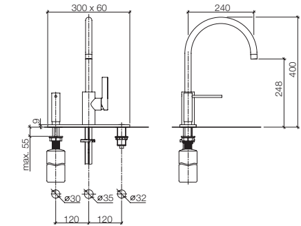
37 858 875 UNI SET Single-lever mixer, 9 1/2" spout projection, with Air Switch (operating button) Miscelatore monocomando, sporgenza 9 1/2", con Air Switch Mezclador monomando, saliente 9 1/2", con Air Switch
