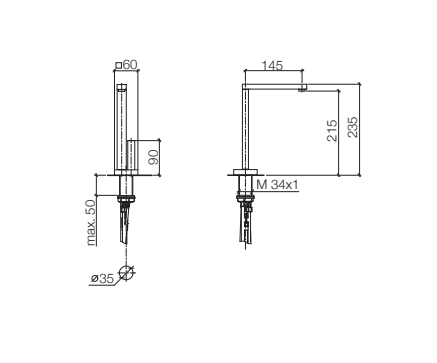
17 851 680 / 17 850 680 Hot & Cold/Hot Water Dispenser, 5 3/4" spout projection Hot & Cold/Hot Water Dispenser, sporgenza 5 3/4" Hot & Cold/Hot Water Dispenser, saliente 5 3/4"
