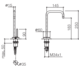
17 851 625 / 17 850 625 Hot & Cold/Hot Water Dispenser, 5 3/4" spout projection Hot & Cold/Hot Water Dispenser, sporgenza 5 3/4" Hot & Cold/Hot Water Dispenser, saliente 5 3/4"
