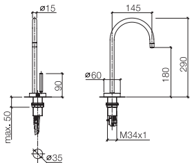
17 851 888 / 17 850 888 Hot & Cold/Hot Water Dispenser, 5 3/4" spout projection Hot & Cold/Hot Water Dispenser, sporgenza 5 3/4" Hot & Cold/Hot Water Dispenser, saliente 5 3/4"
