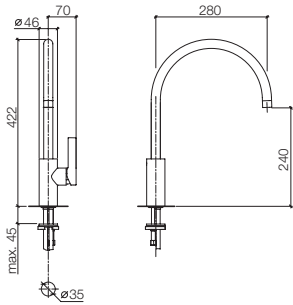
33 818 875 Single-lever mixer, 11" spout projection Miscelatore monocomando, sporgenza 11" Mezclador monomando, saliente 11"
