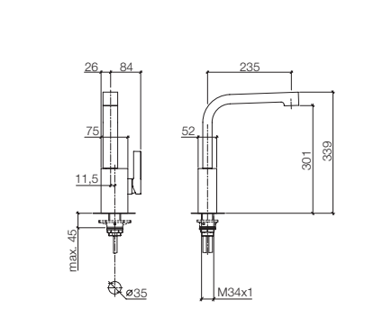
33 800 795 Single-lever mixer, 9 1/4" spout projection Miscelatore monocomando, sporgenza 9 1/4" Mezclador monomando, saliente 9 1/4"
