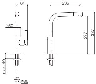
33 800 790 Single-lever mixer, 9 1/4" spout projection Miscelatore monocomando, sporgenza 9 1/4" Mezclador monomando, saliente 9 1/4"
